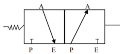
VALVE POSITION 1 2
